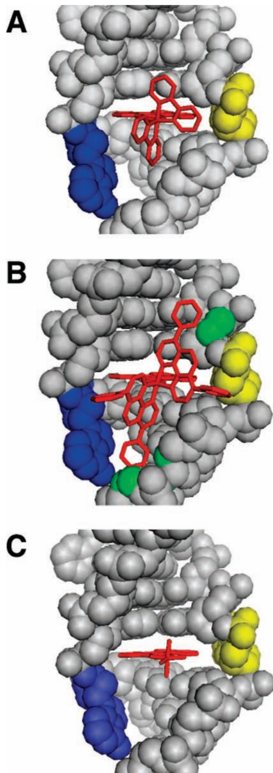
Figure 7. Crystal and model structures of rhodium metalloinsertors bound to the mismatch site. Rhodium insertors (red) are shown bound to the DNA (gray) from the minor groove at the mismatch site with the bases (adenine in blue, cytosine in yellow) ejected and the chrysi ligand stacked fully with the adjacent base pairs. The crystal structure of \Delta\text{-Rh}(\text{bpy})_2\text{chrysi}^{3+} bound to the CA mismatch is shown in panel (A), along with structural models of \Delta\text{-Rh}(\text{DIP})_2\text{chrysi}^{3+} (B) and \Delta\text{-Rh}(\text{NH}_3)_4\text{chrysi}^{3+} (C) binding based on the crystal structure. Superposition of the DIP complex upon the rhodium center of the bpy complex leads to steric clashes with the sugar–phosphate backbone (possible atoms involved in green), whereas the tetraammine complex is easily accommodated.
