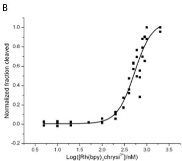
Figure 2. Binding affinities determined through DNA photocleavage. The DNA hairpin sequence is 5'-GGCAGG X ATGGCTTTTTGCCATCCCT-GCC-3' (X = C or A, underline denotes the mismatch). Samples were irradiated and electrophoresed through a 20% denaturing PAGE gel. A light control (LC, without rhodium) and dark control (DC, without irradiation) were included. A representative autoradiogram of a photocleavage titration with rac -Rh(bpy) 2 chrysi 3+ (A, arrows indicate positions of mismatched bases) and a representative sigmoidal curve fit of pooled data from photocleavage titrations for binding constant determination (B) are shown.
